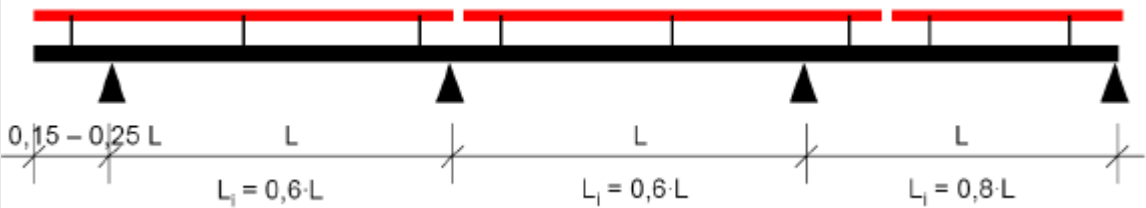
Figure 11: Equivalent support spacing
