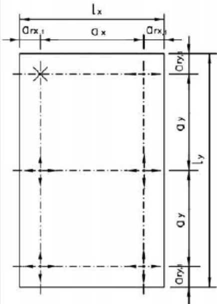
Figure 13: Façade panel with 6 agraffes – support condition 2
