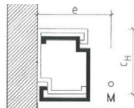
Figure 8: Open profile with shear centre
