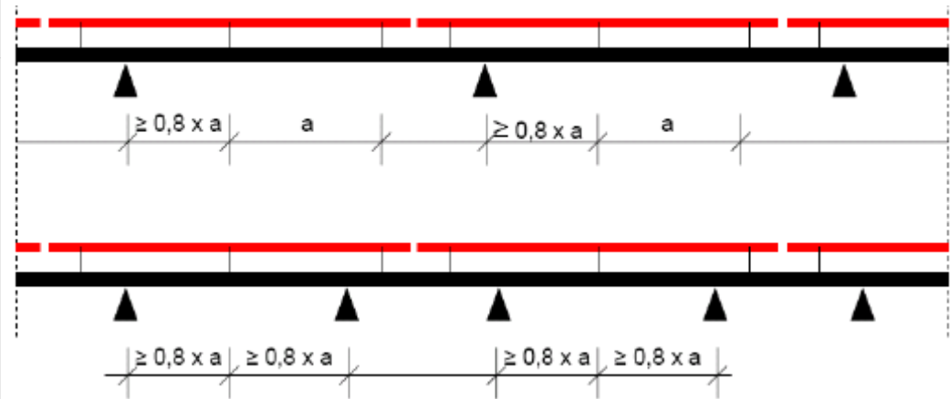
Figure 10: In profiles, supporting three fixing points of a panel, the central fixing points must have a minimum distance of 0,8 x a (a= spacing of the fixing points of the panel) to the supports.
