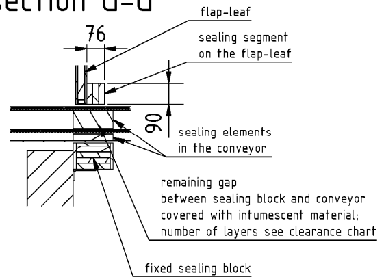
section G-G
