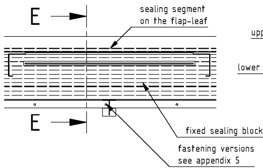
schematic diagram sealing of roller conveyor
