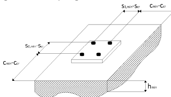
Scheme of edge distance and spacing in concrete
