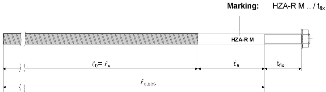
Figure A7: Hilti tension anchor HZA-R
