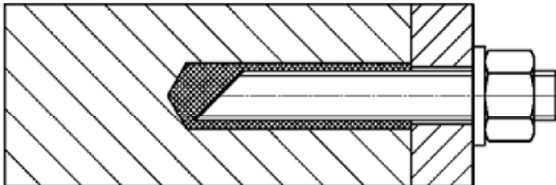
Standard threaded rod with two side 45° chamfer
