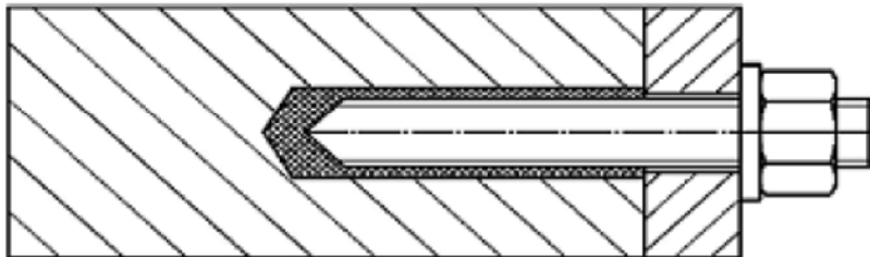
Standard threaded rod with two side 45° chamfer
