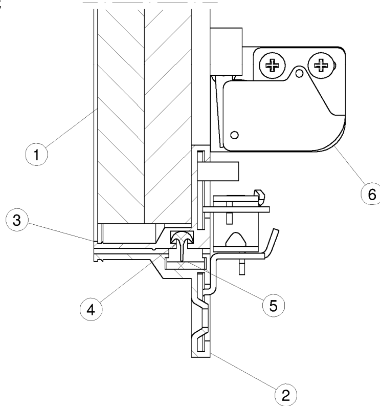
Detail B
