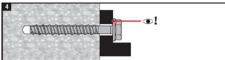
4 Ensure that the head of the anchor is fully supported on the fixture and it is not damaged.
