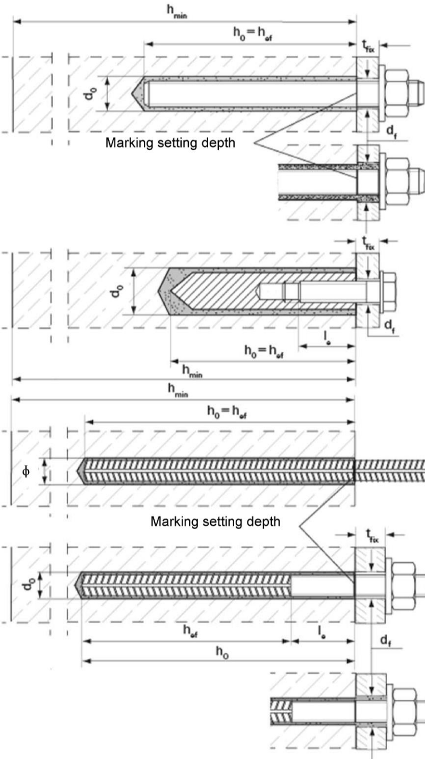
Anchor rod UVT Top A pre-positioned anchorage
