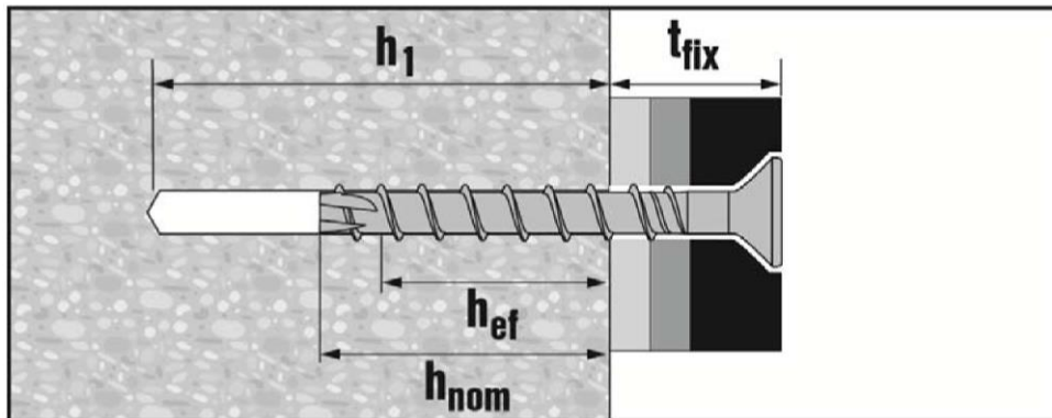
HUS3-C (countersunk head configuration sizes 8 and 10 – h_{nom2} )
