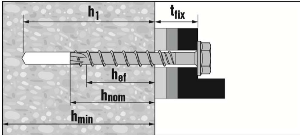
HUS3-H (hexagon head configuration sizes 8 and 10 – h_{nom2} )
