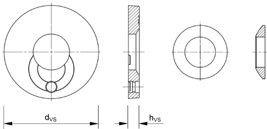
Sealing washer
