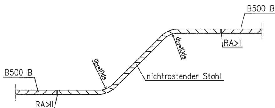
Diagonalstabvariante 1
