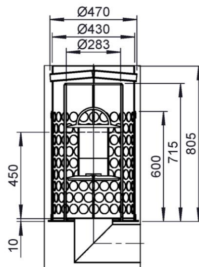
Detail Z
