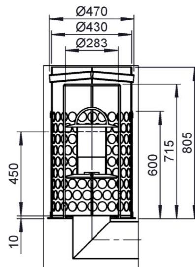
Detail Z
