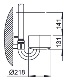
Detail Z
