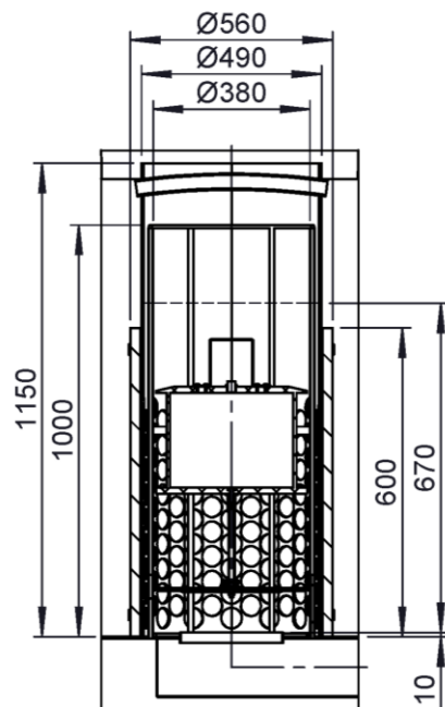
Detail Z
