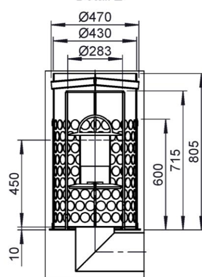
Detail Z
