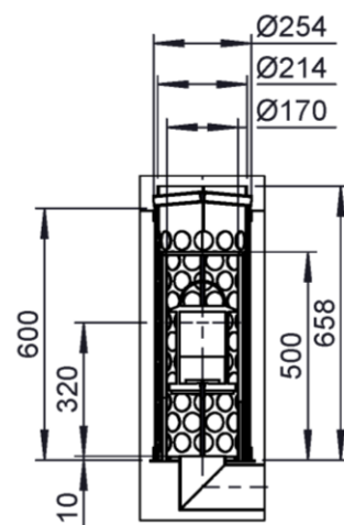
Detail Z
