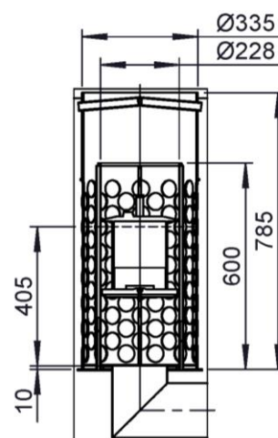
Detail Z
