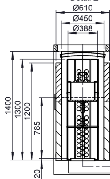
Detail Z
