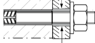
fischer rebar anchor FRA Push through anchor (annular gap filled with mortar)
