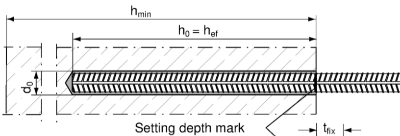
Reinforcing bar
