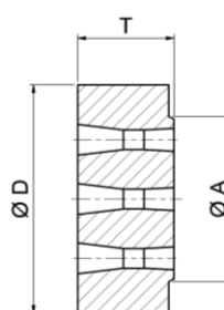
Anchor Head
