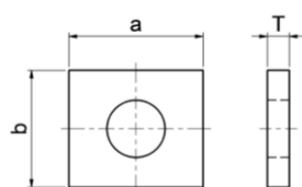
Bearing Plate, rectangular
