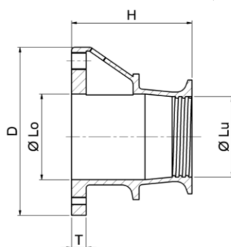
Cast-iron Anchor Body
