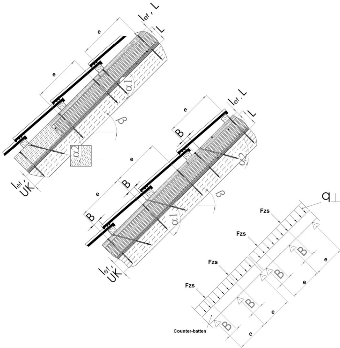
Figure A.5.4 Fastening of thermal insulation material on top of rafters - structural system for alternatively inclined screws and continuous batten under constant line loads from actions on the roof plane q_{\perp} and concentrated loads from tensile screws F_{zs}
