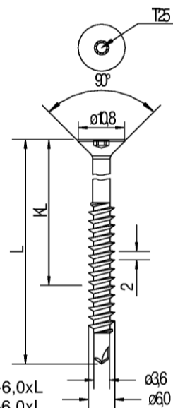
JT3-ST-2-6,0 x L JT2-ST-2-6,0 x L
