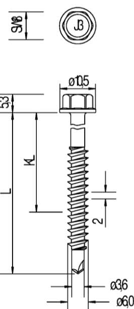
JT3-ST-2-6,0 x L JT2-ST-2-6,0 x L
