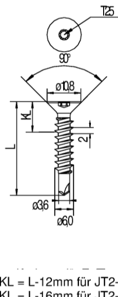
JT3-ST-2-6,0 x L JT2-ST-2-6,0 x L
