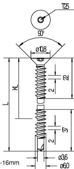
JT3-ST-2-6,0 x L / UG
