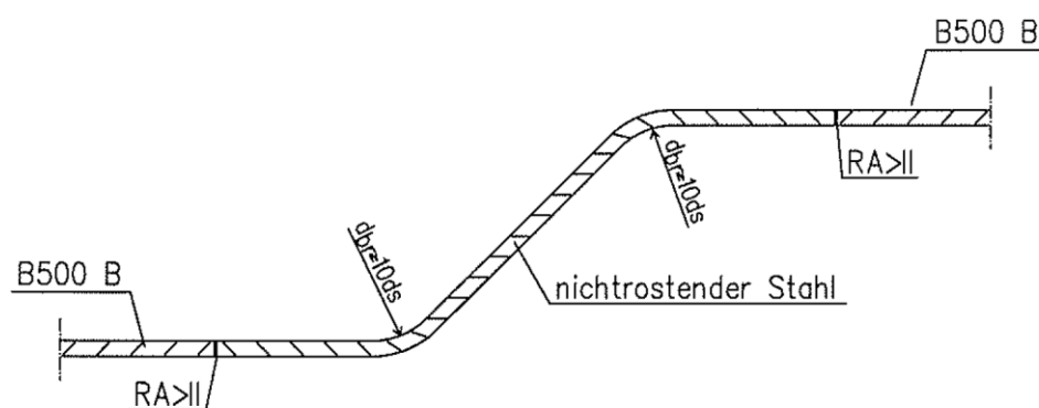
Diagonalstabvariante 1
