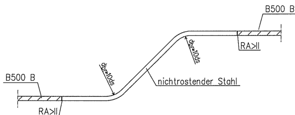
Diagonalstabvariante 2
