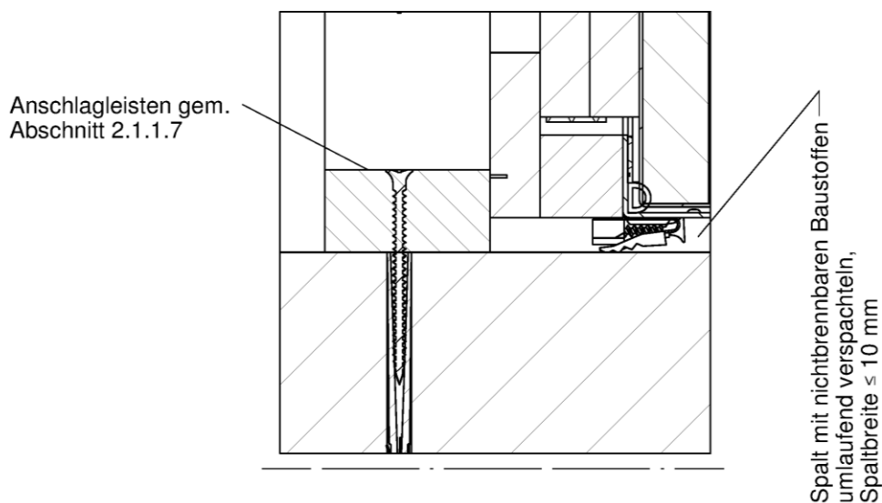
Detail I
