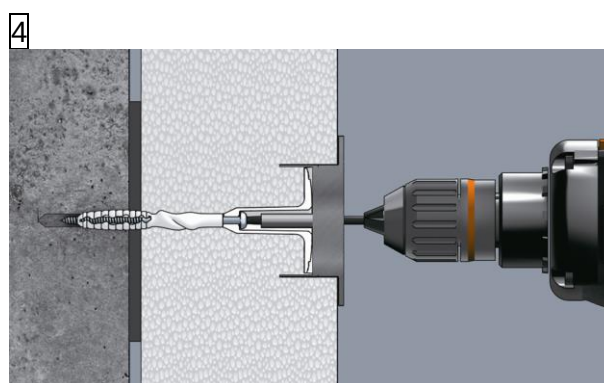
Countersunk installation with STR-tool
