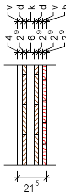
Wall type 21,5 vertical
