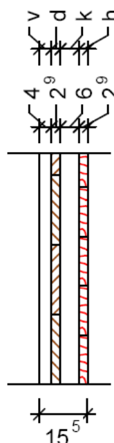
Wall type 15,5 vertical
