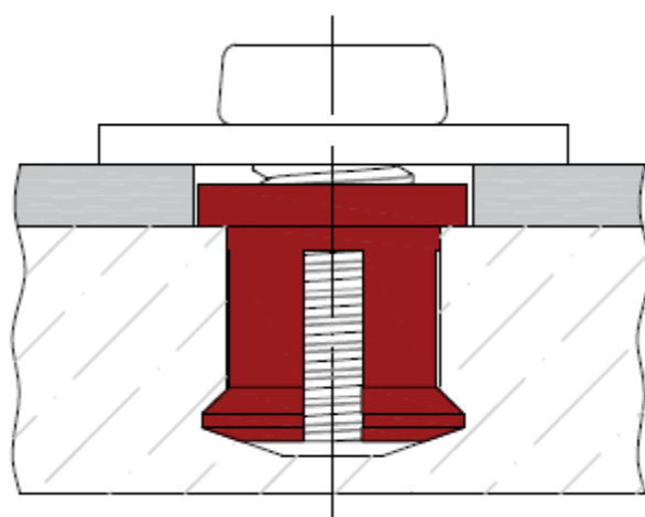
b) Installed undercut anchor
