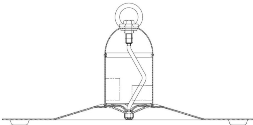
Constant Force Post Intermediate CFP Int.
