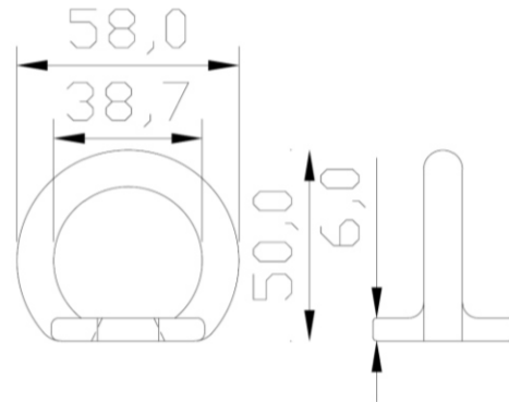
85030-00 D-Ring
