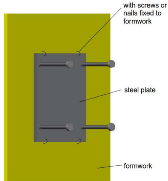
Fig. 3: steel plate fixed to the formwork
