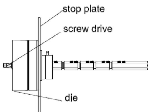
Mounting tool
