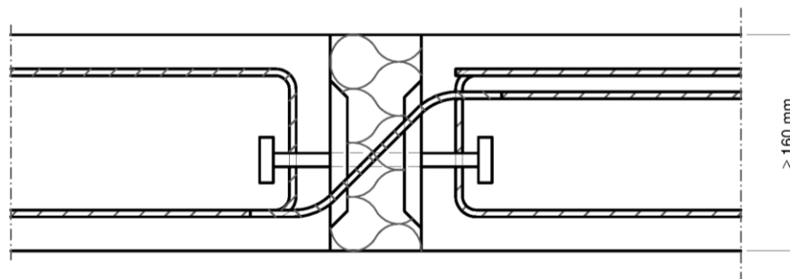
Fig. 14 Example of a Schöck Isokorb® type Q with SCE with on-site reinforcement
