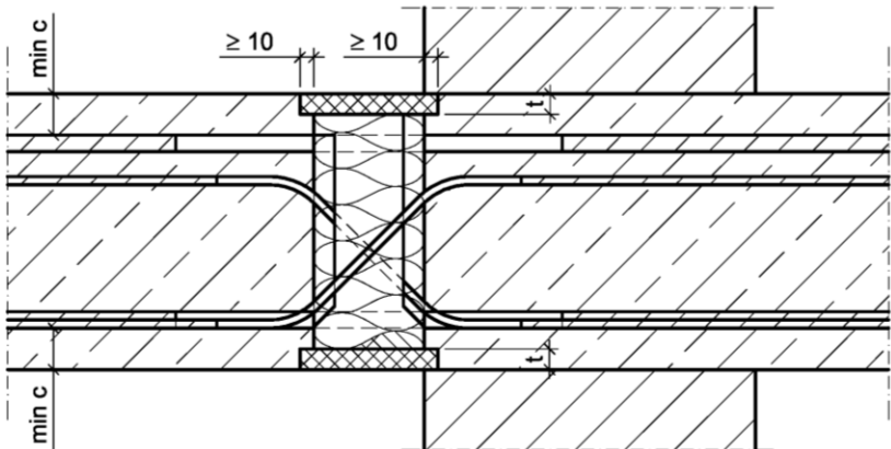
Fig. 22 Schöck Isokorb® type D with SCE
