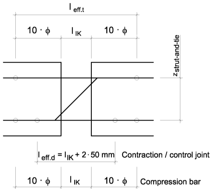
Fig. 36 l_{eff} for ribbed stainless steel bar, as per section A.3
