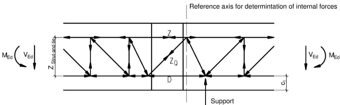
Fig. 25 Schöck Isokorb® type K and KF (version segmented)
