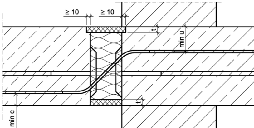
Fig. 23 Schöck Isokorb® type Q and type QF
