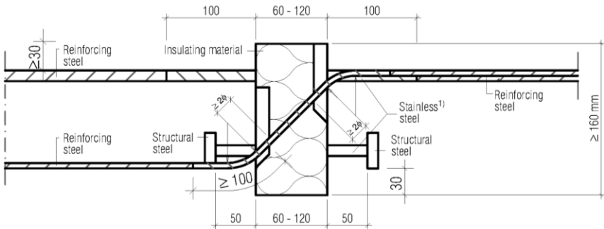
Fig. 10 Schöck Isokorb® type K with SCE
