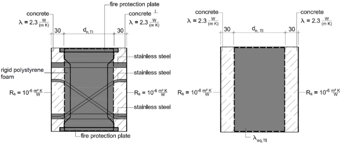
Fig. 24 cross section of configuration to calculate the equivalent thermal resistance R_{eq,TI} and simplified analogous model with \lambda_{eq,TI}
