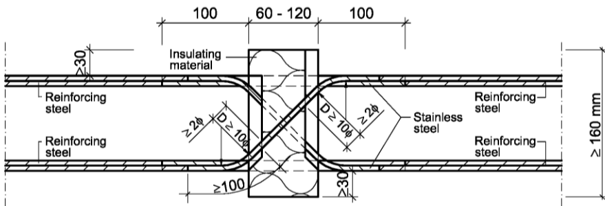
Fig. 16 Schöck Isokorb® type D with SCE
