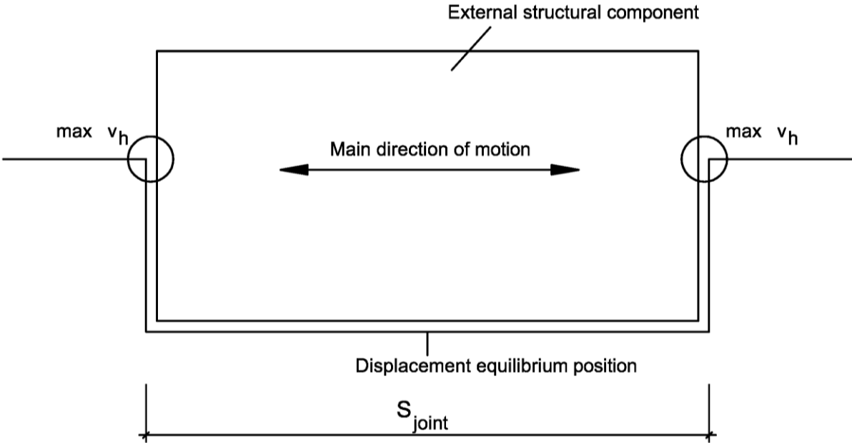
Fig. 8 Installation situation with support on opposite edges
