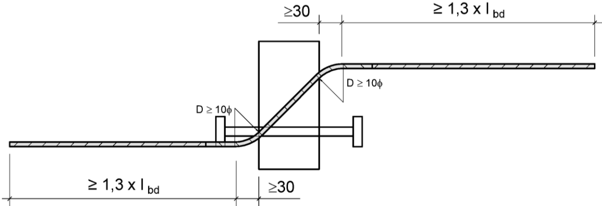
Fig. 30 Schöck Isokorb® type K / KF (version segmented)
