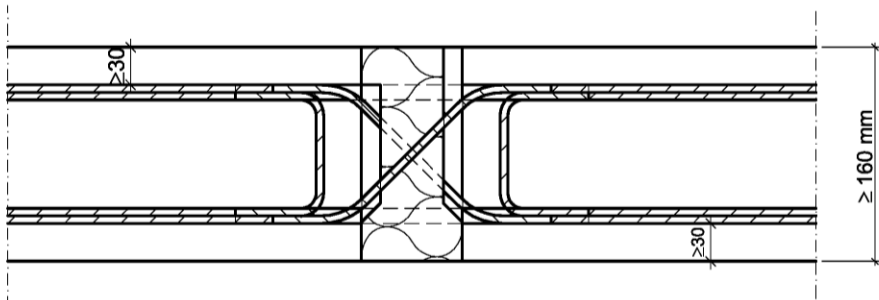
Fig. 17 Example of a Schöck Isokorb® type D with SCE with on-site reinforcement
