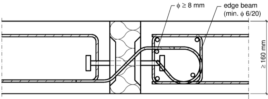
Fig. 34 Example for a Schöck Isokorb® type Q with SCE and execution as edge beam
