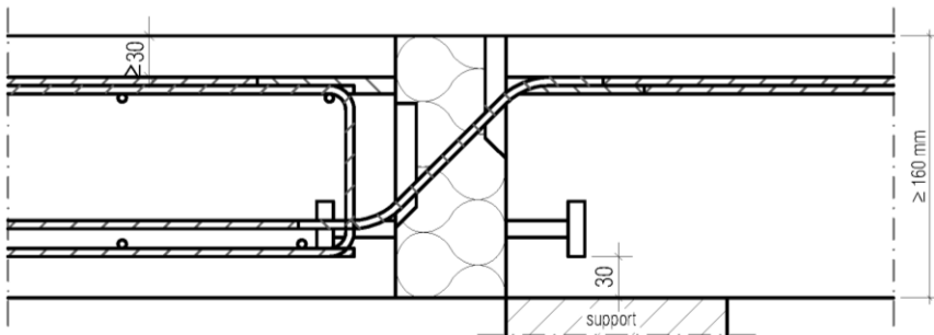
Fig. 12 Example of a Schöck Isokorb® type K with SCE with on-site reinforcement
