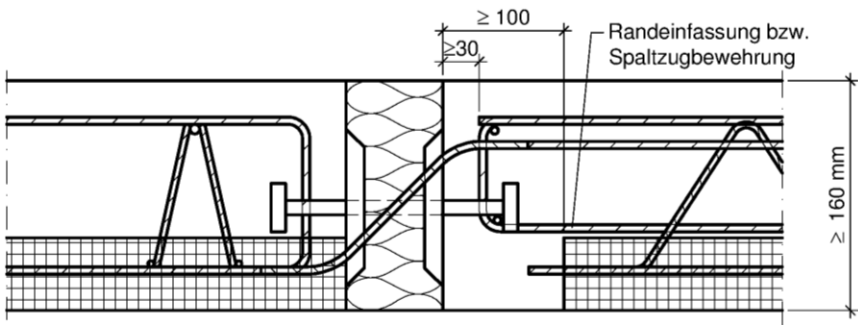
Fig. 19 Example of a Schöck Isokorb® type Q with prefabricated concrete slabs
