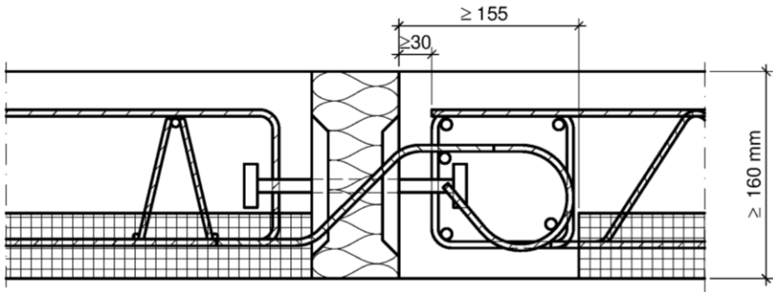
Fig. 20 Example of a Schöck Isokorb® type Q with prefabricated concrete slabs
