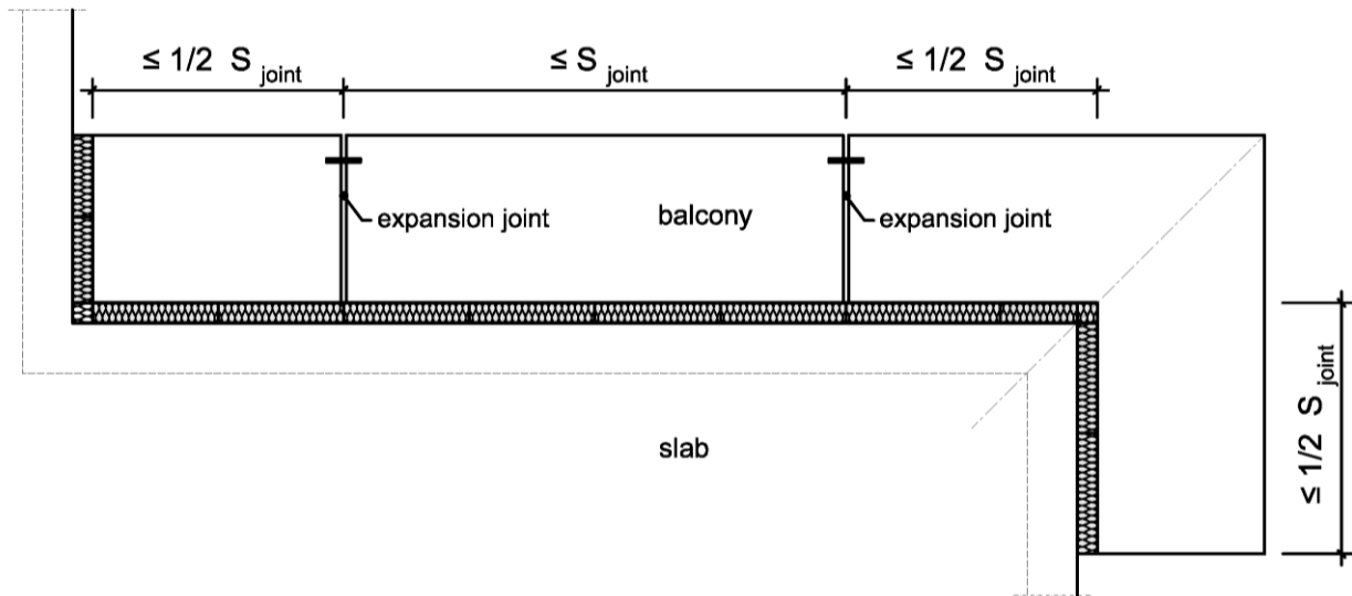
Fig. 9 Installation situation with expansion joint
