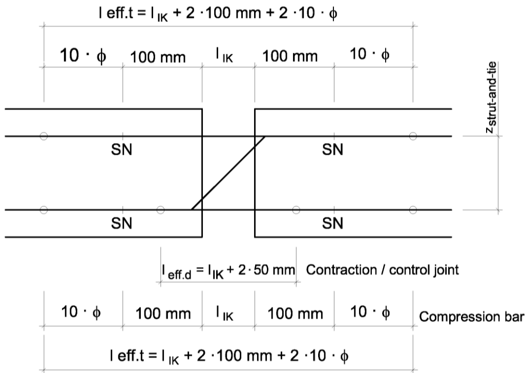
Fig. 37 l_{eff} for plain stainless steel bar with strength classes S 355, S 460 and S 690, as per section A.3
