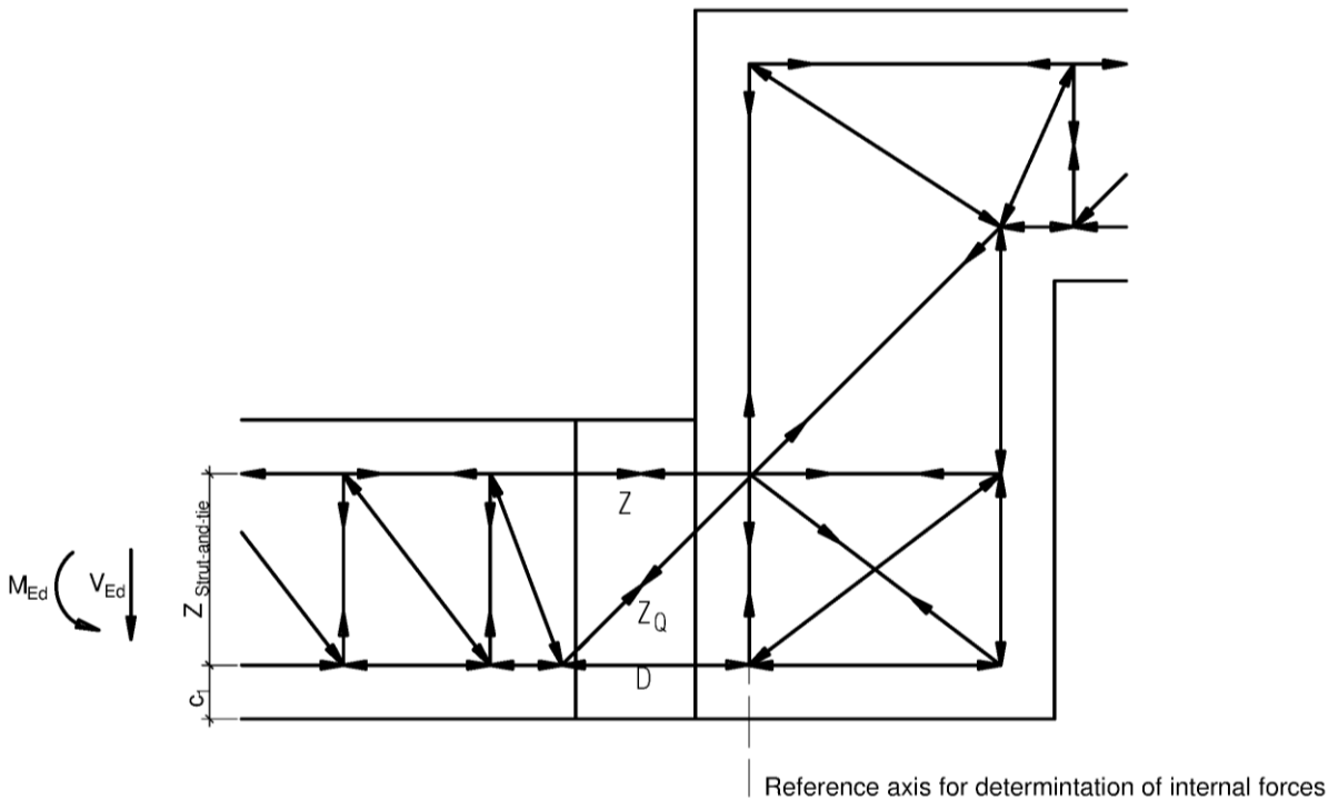
Fig. 26 Schöck Isokorb® type K (high offset variant)
