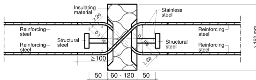
Fig. 15 Schöck Isokorb ® type Q+Q with SCE
