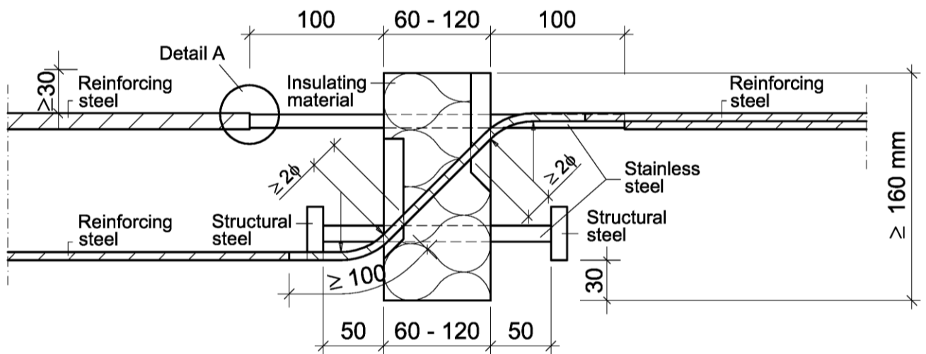
Fig. 6 Schöck Isokorb® type K with SCE
