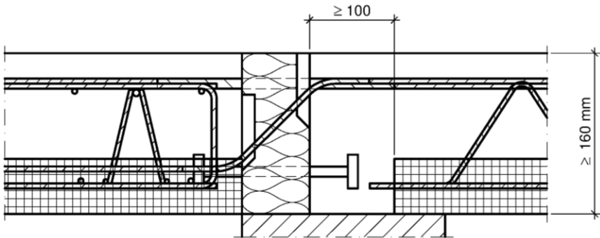
Fig. 18 Example of Schöck Isokorb® type K or KF (Version segmented) with prefabricated concrete slabs
