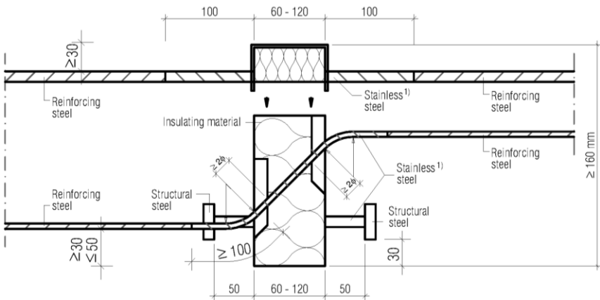
Fig. 11 Schöck Isokorb® type KF (version segmented) with SCE
