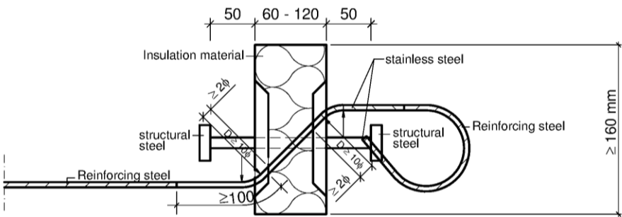
Fig. 33 Schöck Isokorb® type Q with SCE
