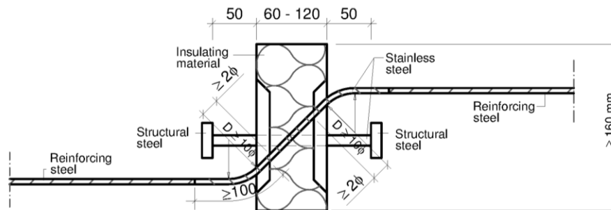
Fig. 13 Schöck Isokorb® type Q with SCE
