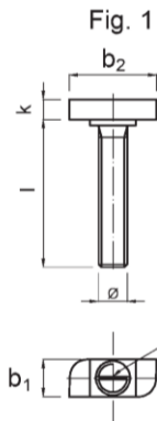
Hammer-head channel bolt
