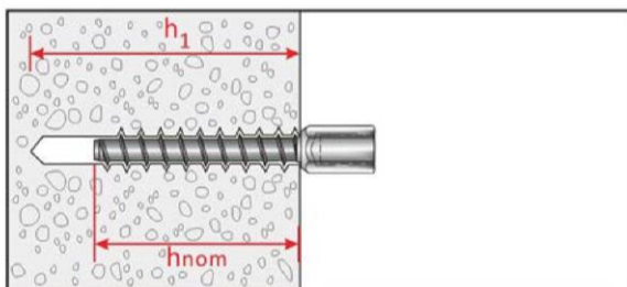
Hanger Bolt : SASS A4 (SA10-M12)
