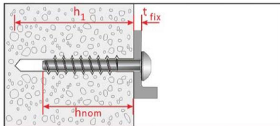
Button Head : SAB 10B21 (SA8, SA10) A4 (SA8, SA10)
