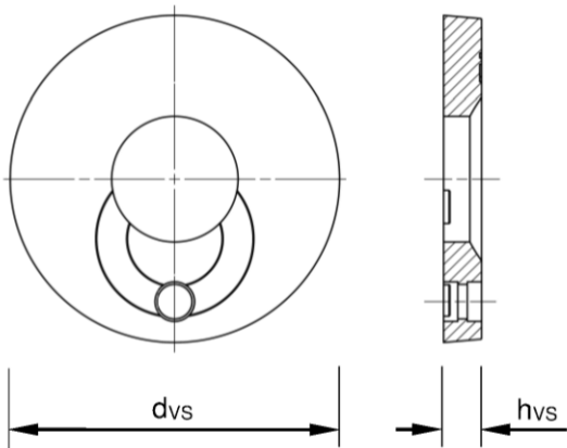
Sealing washer
