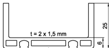
DL 5061, Aluminium
