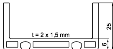
DL 5061, Aluminium
