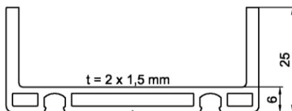
DL 6061, Aluminium
