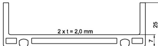
DL 8061, Aluminium
