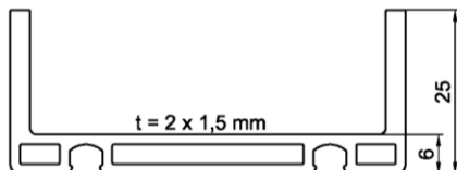
DL 6061, Aluminium
