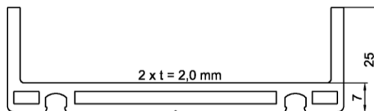
DL 8061, Aluminium
