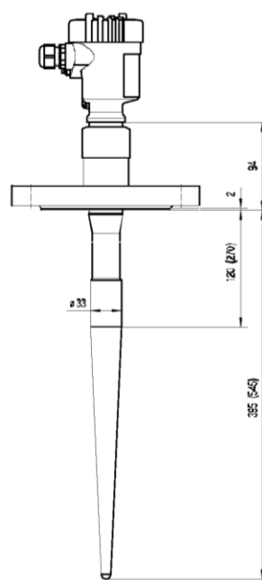
VEGAPULS63
