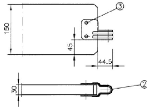
Detail Z
