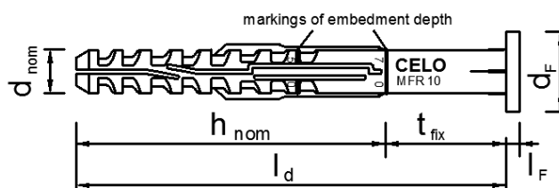
MFR 10 FB (alternative)
