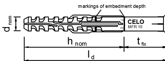
MFR 10 SB (alternative)
