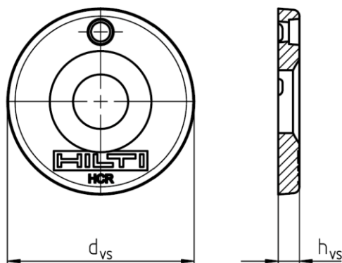
Sealing washer
