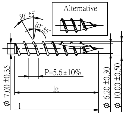
Quickdrill II
