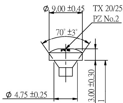
Pan Head
