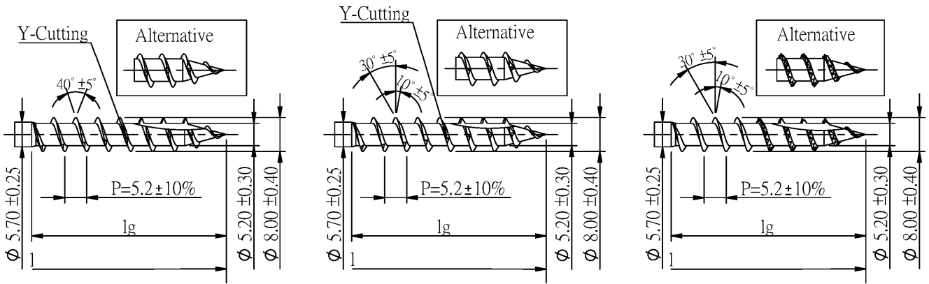
Quickdrill
