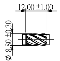
Shank cutter
