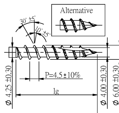
Quickdrill II
