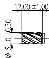
Shank cutter
