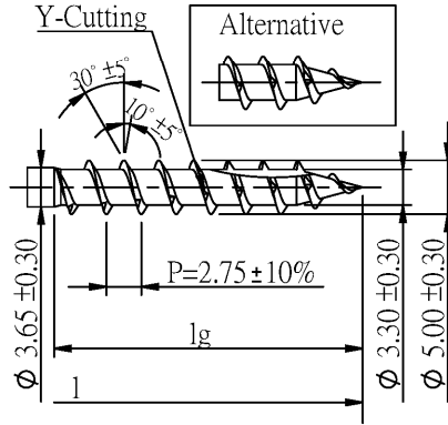
Quickdrill +
