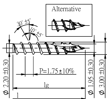
Quickdrill III
