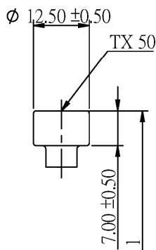
Cylinder Head
