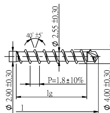
Quickdrill DP+
