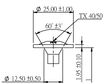
Wafer Head
