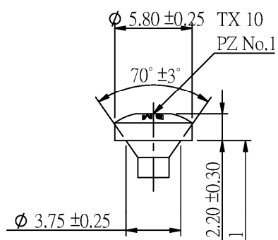
Pan Head
