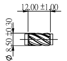
Shank cutter
