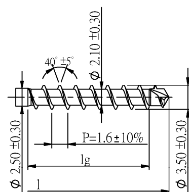
Quickdrill DP+
