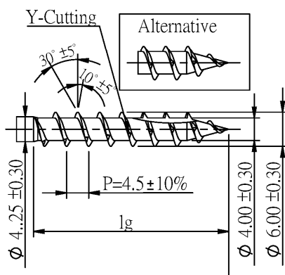
Quickdrill +
