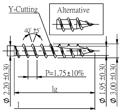
Quickdrill
