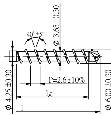
Quickdrill DP+
