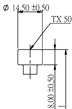
Cylinder Head
