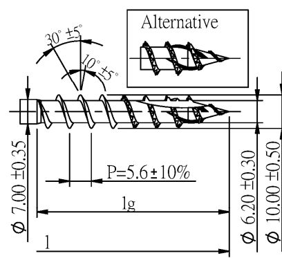
Quickdrill III
