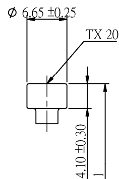
Cylinder Head
