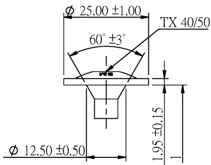
Wafer Head
