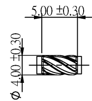
Shank cutter
