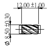
Shank cutter
