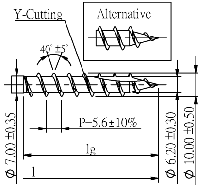
Quickdrill
