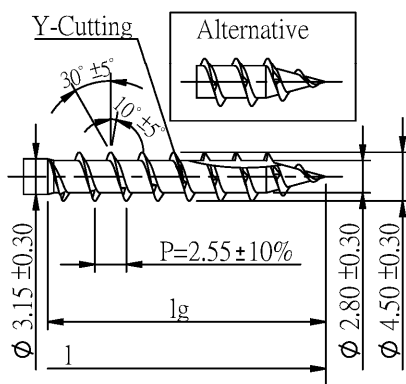
Quickdrill +
