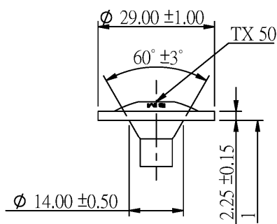
Wafer Head
