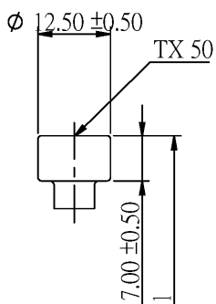
Cylinder Head
