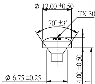
Pan Head
