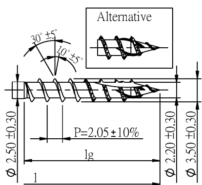
Quickdrill III
