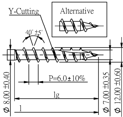
Quickdrill
