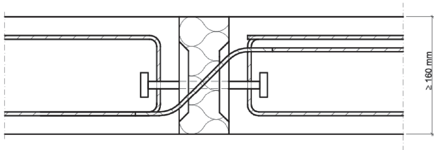
Fig. 19 Example of a Schöck Isokorb® type Q with SCE with on-site reinforcement
