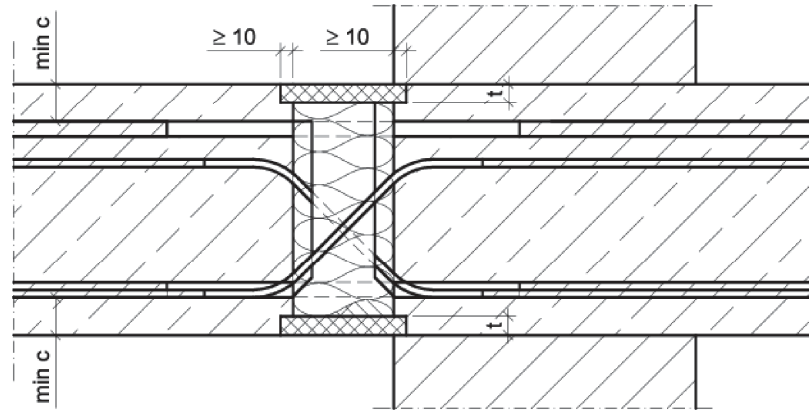
Fig. 31 Schöck Isokorb® type D (analog A and F) with SCE
