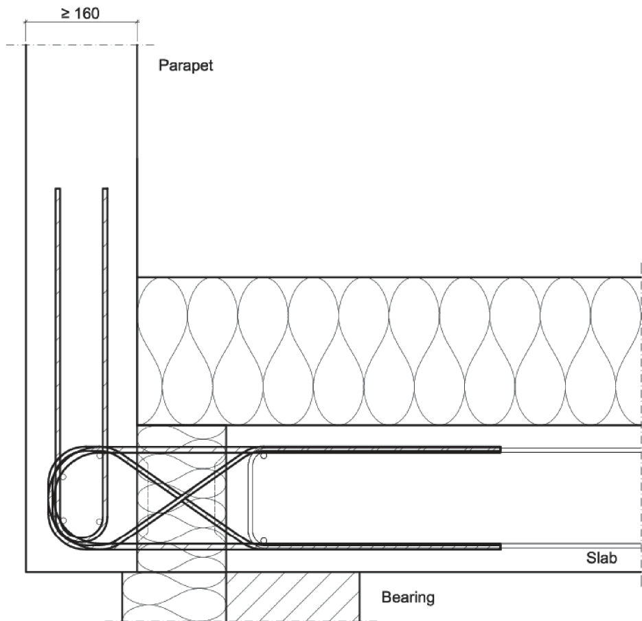
Fig. 26 Example of a Schöck Isokorb® type F with SCE with on-site reinforcement
