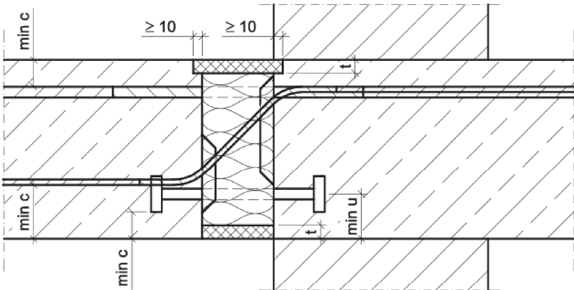
Fig. 30 Schöck Isokorb® type K and KF (analog O) with SCE
