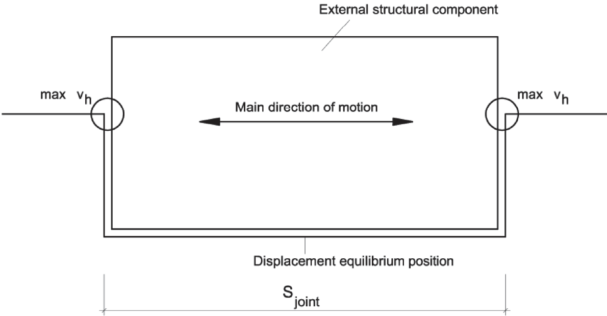
Fig. 11 Installation situation with support on opposite edges
