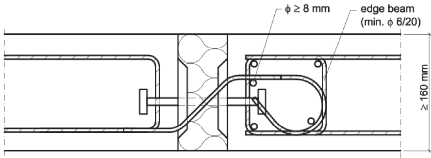
Fig. 46 Beispiel Schöck Isokorb® type Q type Q with SCE and execution as edge beam
