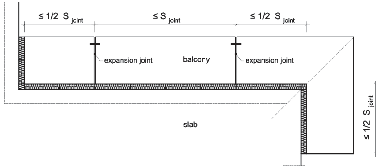
Fig. 12 Installation situation with expansion joint
