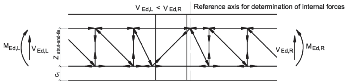
Fig. 38 Schöck Isokorb® type D (type A and F analog)
