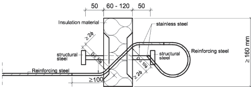
Fig. 45 Schöck Isokorb® type Q with SCE
