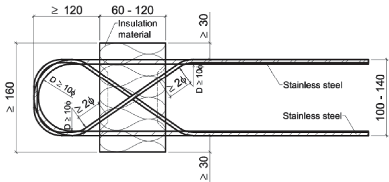
Fig. 25 Schöck Isokorb® type F with SCE
