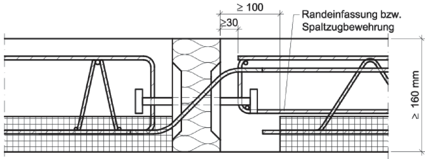
Fig. 28 Example of a Schöck Isokorb® type Q with prefabricated concrete slabs
