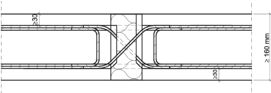
Fig. 22 Example of a Schöck Isokorb® type D with SCE with on-site reinforcement
