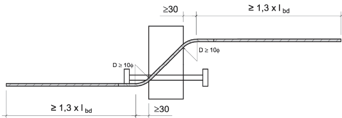
Fig. 39 Schöck Isokorb® type K/KF (version segmented)
