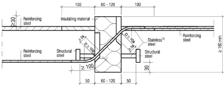
Fig. 13 Schöck Isokorb® type K with SCE
