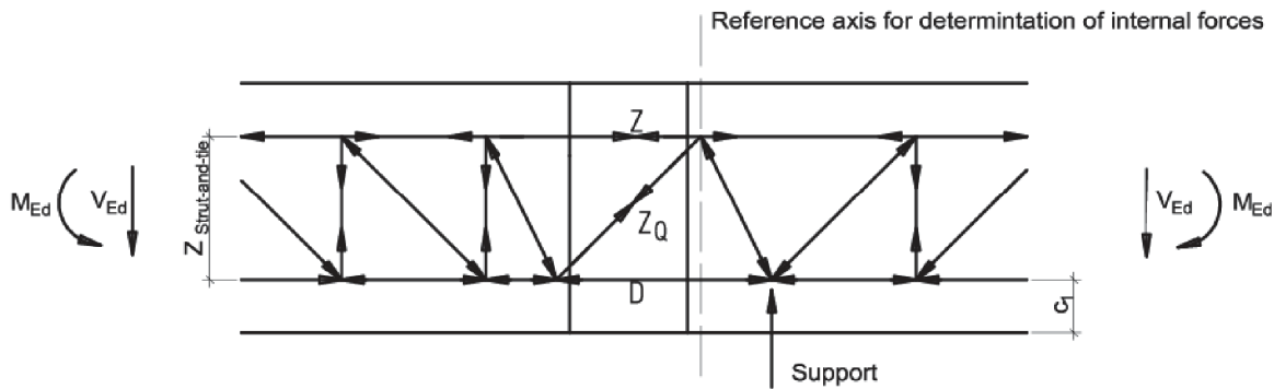
Fig. 34 Schöck Isokorb® type K and KF (version segmented) (type O analog)
