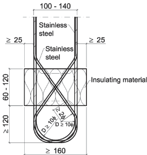
Fig. 23 Schöck Isokorb® type A with SCE
