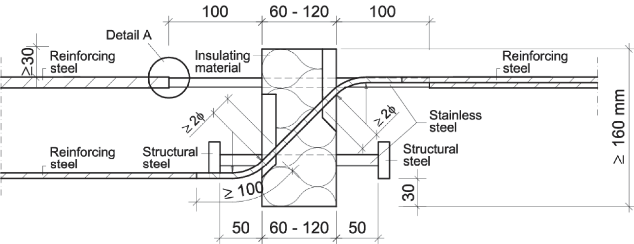
Fig. 9 Schöck Isokorb® K with SCE
