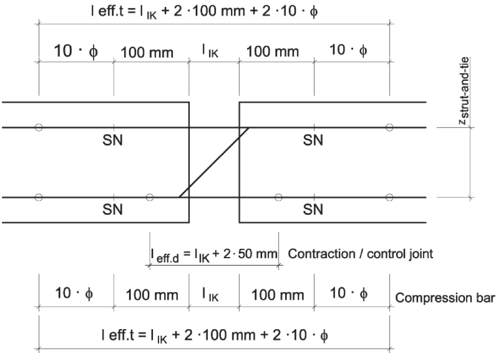
Fig. 49 l_{eff} for plain stainless steel bar with strength classes S 355, S 460 and S 690, as per sect. A.3
