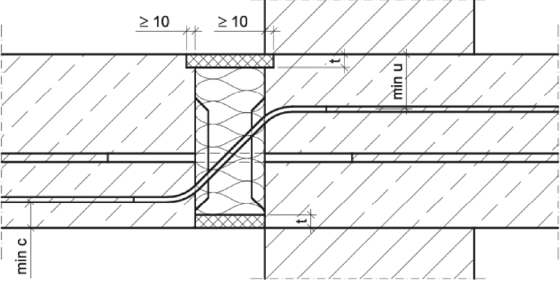
Fig. 32 Schöck Isokorb® type Q with SCE
