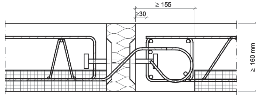
Fig. 29 Example of a Schöck Isokorb® type Q with prefabricated concrete slabs
