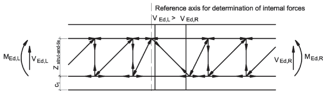
Fig. 37 Schöck Isokorb® type D (type A and F analog)
