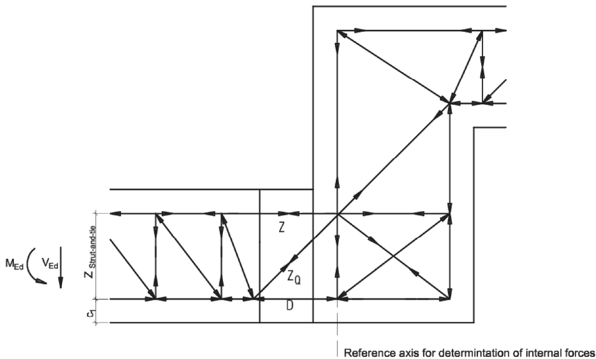
Fig. 35 Schöck Isokorb® type K (high offset variant)
