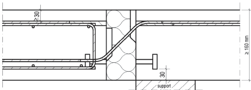
Fig. 15 Example of a Schöck Isokorb® type K with SCE with on-site reinforcement
