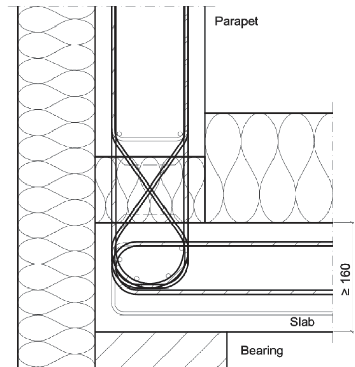
Fig. 24 Example of a Schöck Isokorb® type A with SCE with on-site reinforcement
