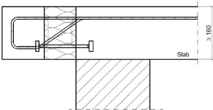
Fig. 17 Example of a Schöck Isokorb® type O
