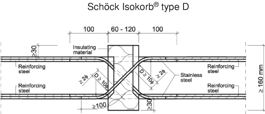
Fig. 21 Schöck Isokorb® type D with SCE
