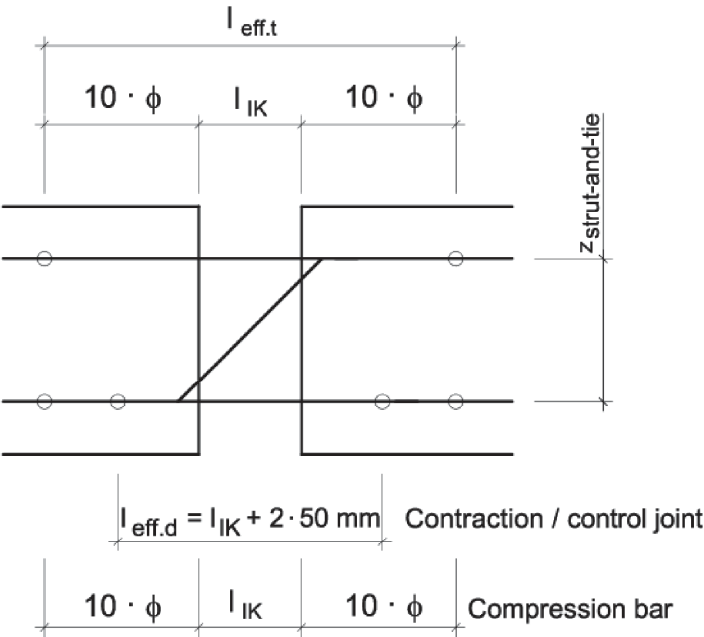
Fig. 48 l_{eff} for ribbed stainless steel bar, as per section A.3
