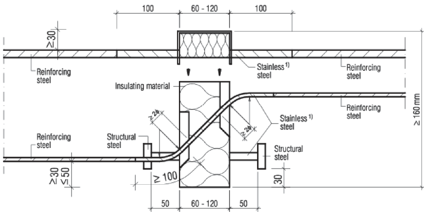
Fig. 14 Schöck Isokorb® type KF (version segmented) with SCE
