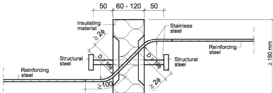
Fig. 18 Schöck Isokorb® type Q with SCE
