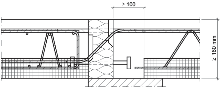
Fig. 27 Example of a Schöck Isokorb® type K and KF (Version segmented) with prefabricated concrete slabs
