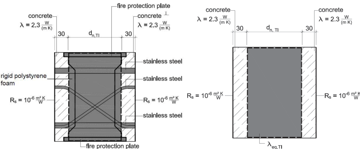
Fig. 33 cross section of configuration to calculate the equivalent thermal resistance R_{eq,TI} and simplified analogous model with \lambda_{eq,TI}
