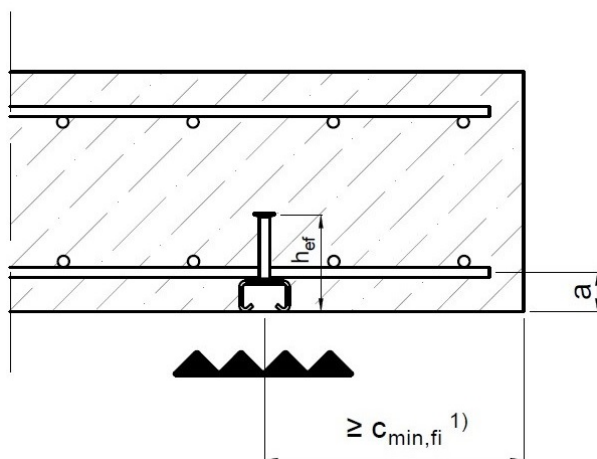
Fig. 1 One sided fire exposure
