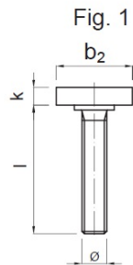
Hammer-head channel bolt
