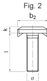
Hook-head channel bolt
