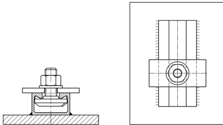
Figure 1: Principle setup of hot-rolled mounting channel
