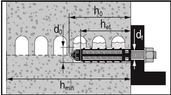
Figure A1: Hollow brick with HAS-U-... and one sieve sleeve HIT-SC (see Table B5)
