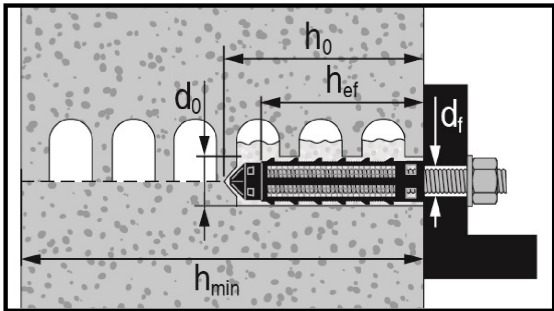
Figure A1: Hollow brick with HAS-U-... and sieve sleeve HIT-SC (see Table B5)
