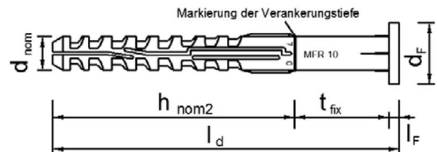
MFR 10 FB (alternative)
