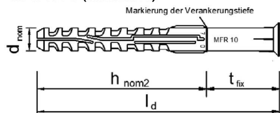
MFR 10 FB (alternative)
