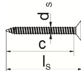
Special screw
