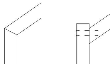
String joint at bottom
