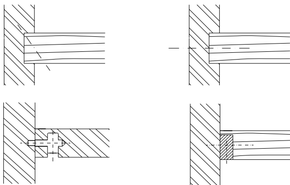
Corner-support of strings
