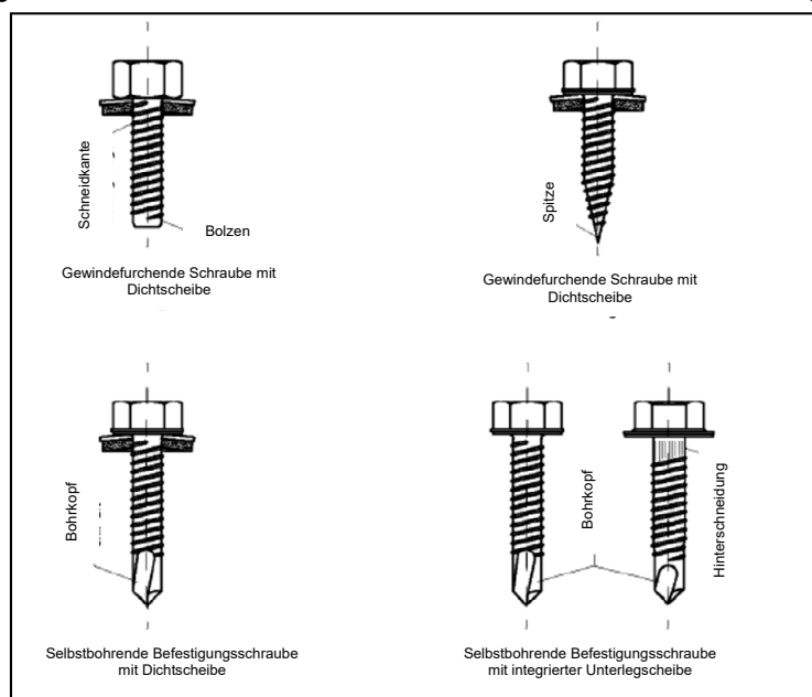
Abbildung 1: Fastening screws
