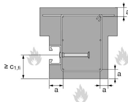
Fire exposure from more than one side
