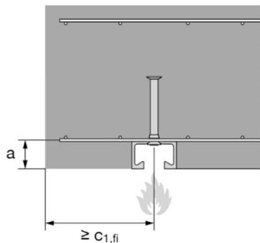
Fire exposure from one side only
