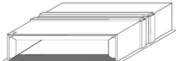
Type 2, threesided, for installation in floors with wall attachment and in walls with attachment to the ceiling, with intumescend strips on the front ends and a circumferential strip in the middle.
