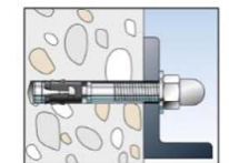
7: Installed fastener
