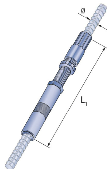
Fig. C8: PH-MU + PH-PA + PH-A
