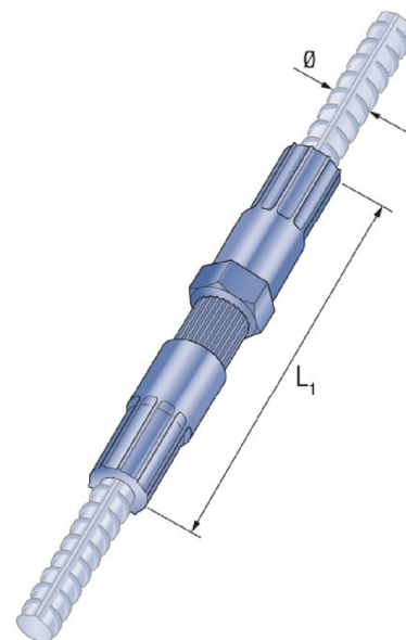
Fig. C4: PH-MU + PH-RL + PH-MU LH
