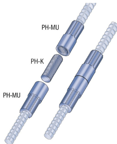
Fig. A2: PH-MU + PH-K + PH-MU
