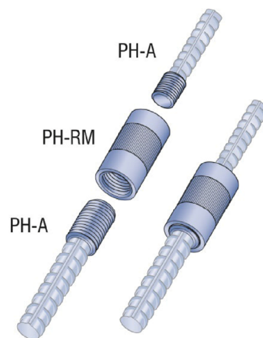
Fig. A6: PH-A + PH-RM + PH-A
