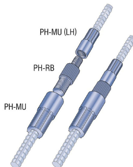
Fig. A5: PH-MU + PH-RB + PH-MU (LH)
