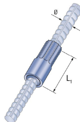
Fig. C1: PH-MU + PH-A
