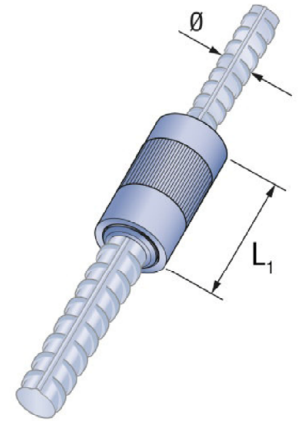
Fig. C6: PH-A + PH-RM + PH-A
