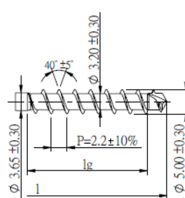
Quickdrill DP+
