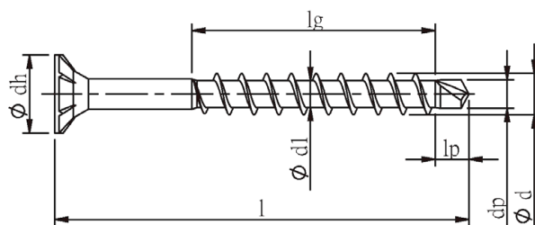
Partial thread with drilling tip
