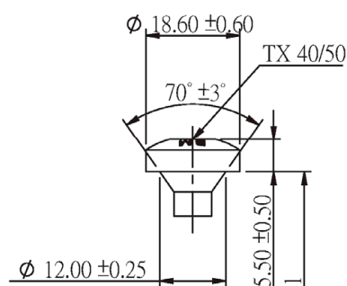
Pan Head
