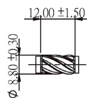
Shank cutter
