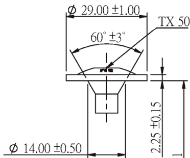
Wafer Head
