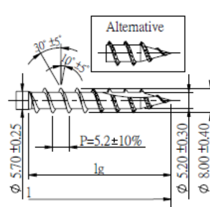
Quickdrill II
