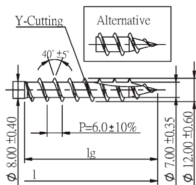
Quickdrill
