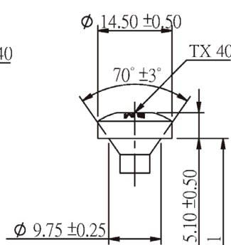
Pan Head
