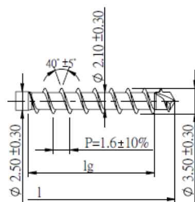
Quickdrill DP+
