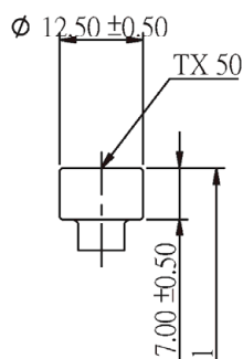
Cylinder Head
