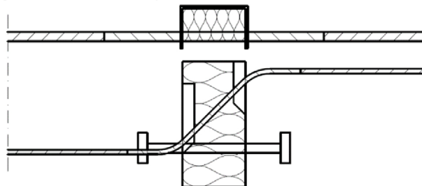
Fig. 2: Schöck Isokorb® type K-F (Variation in several parts)
