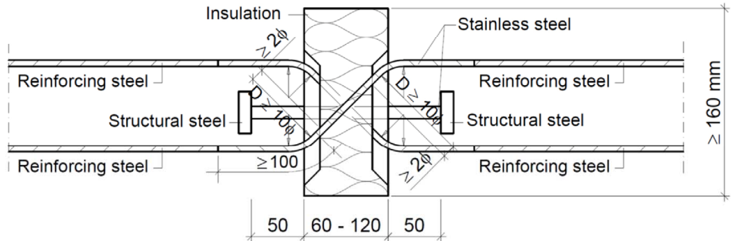
Fig. 22: Schöck Isokorb® type Q-VV with SCE
