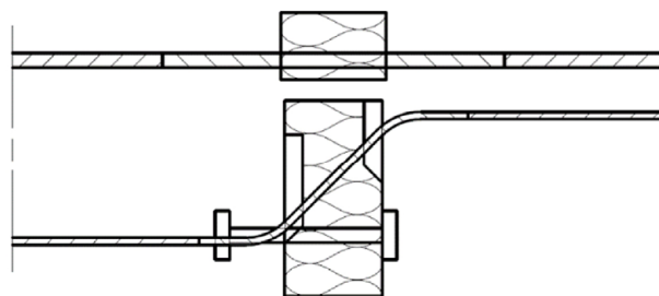
Fig. 4: Schöck Isokorb® type K-ID or RT type K (ceiling side flush compression plates)
